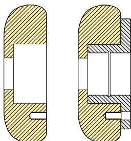
Rulli in Teflon® Rolls made of Teflon®
